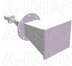
LB-28-25-C2-EKFSPO Standard Gain Horn Antenna 26.5-40GHz 25dB Gain 2.92mm Female
